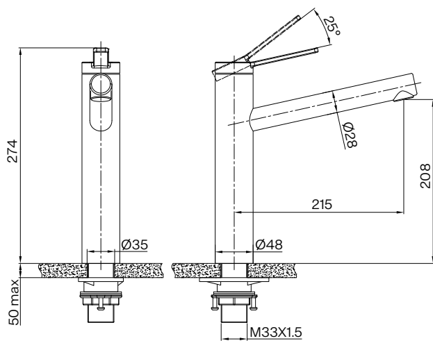
Tap Tango Neo Pull Out Nozzle Top HP SS
